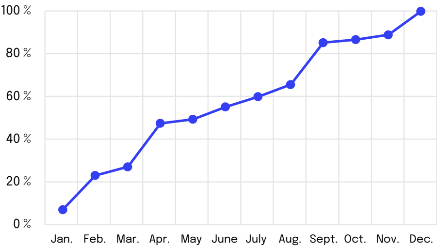
Population living in area having reached Plastic Overshoot Day (%)
