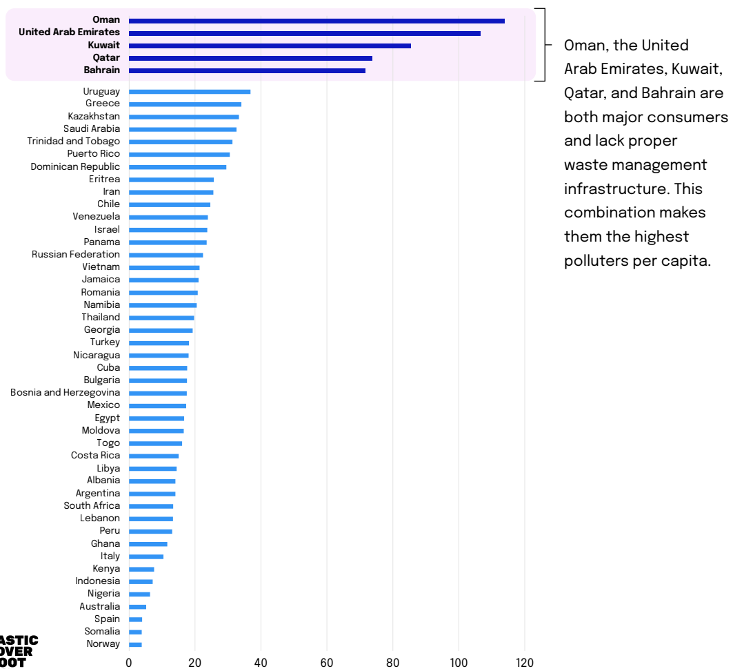
Mismanaged plastic waste per person (kg/capita/year)
